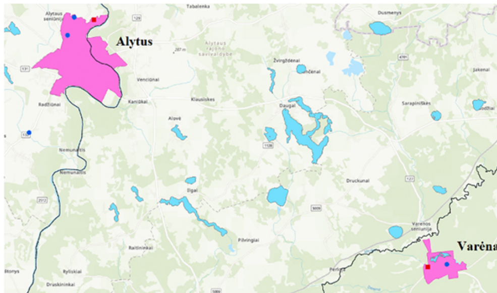
Figure 22. DH area and available heat sources around Alytus, Lithuania
