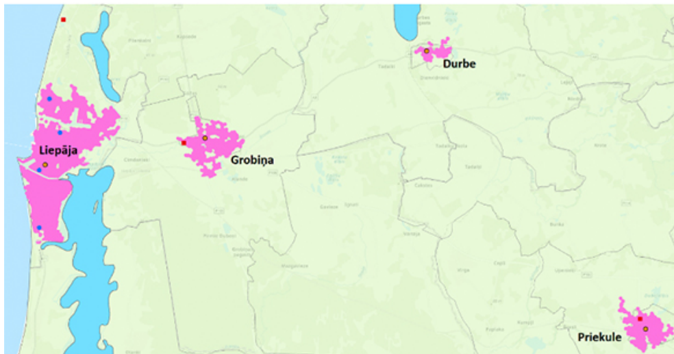
Figure 21. DH area and available heat sources around Liepāja, Latvia
