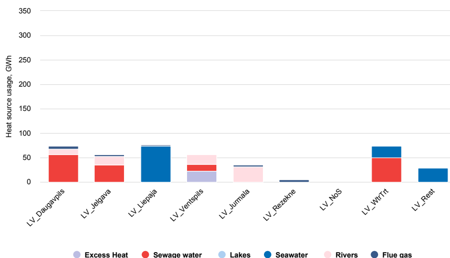
Figure 45. Use of heat sources in Latvia (without Riga) in 2050 according to the Base scenario
