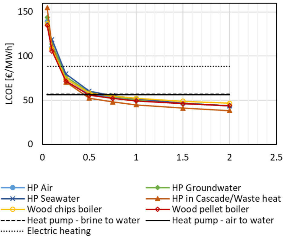
Figure 82. LCOE as a function of the plot ratio for different heat supply options (DH as low-temperature DH (70/40°C), space heating share of 0.13) (copied from 363 )
