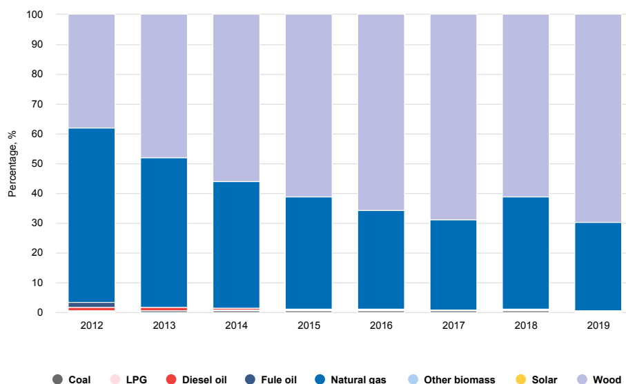
Figure 5. Heat production in Latvia by fuel type 21
