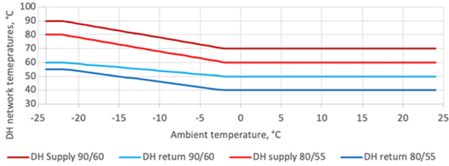
Figure 91. DH supply and return temperatures for two sets of design temperatures
