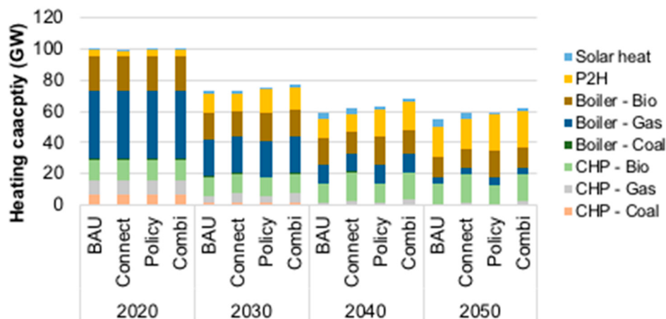
Figure 28. Changes in the energy system at the aggregate level of the Nordic and Baltic countries for the scenarios in 2020-2050. Changes in the heating system (copied from note mangler)
