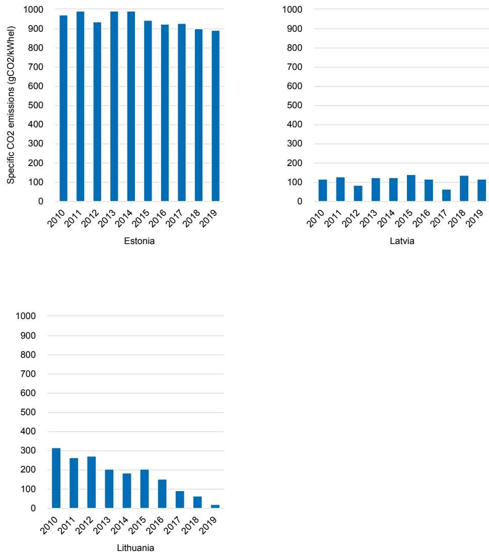
Figure 57. Specific CO 2 emissions for electricity generation 271
