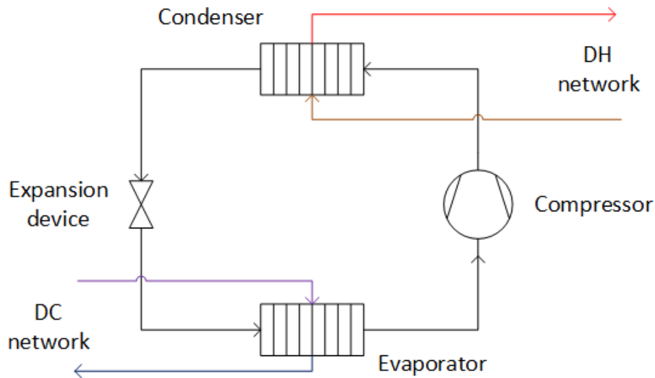
Figure 68. Main components of HP supplying DH and DC (copied from 325 )
