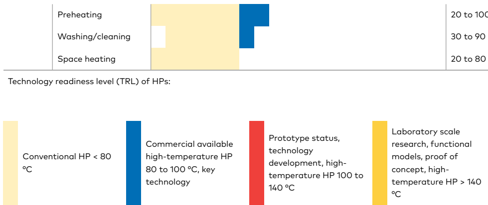
Figure 89. Overview of processes and their typical temperature range in different industrial as well as the Technology Readiness Level of industrial HPs, based on 388
