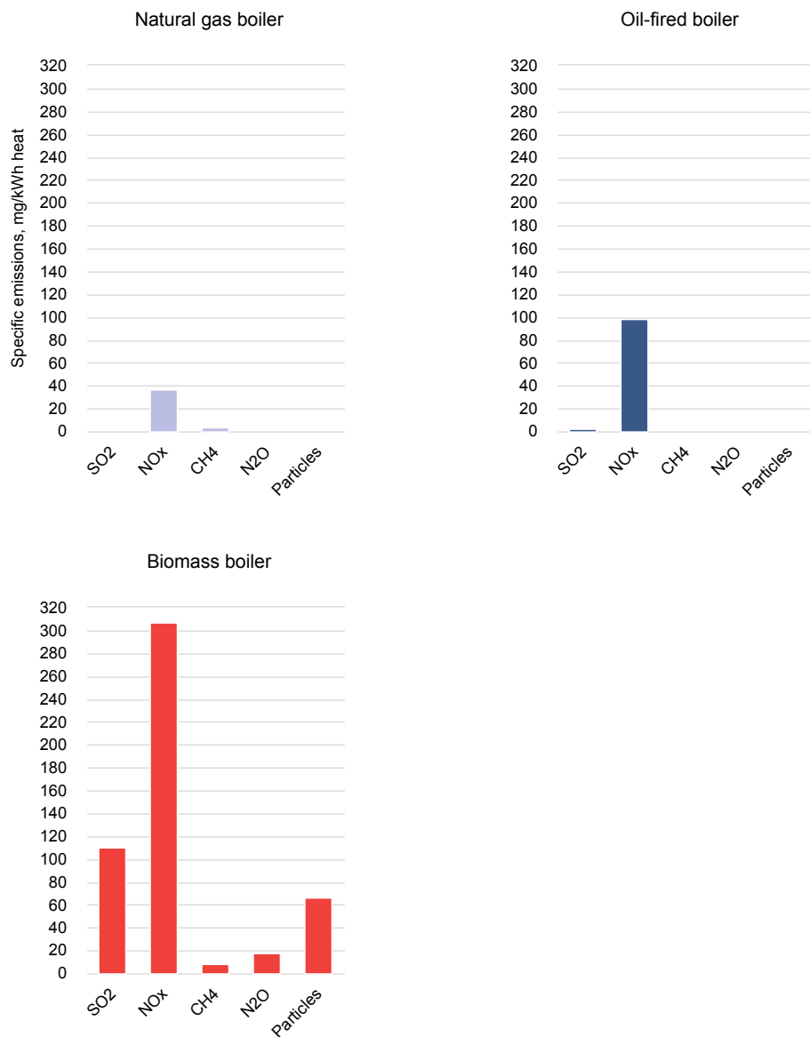
Figure 80. Specific emissions for individual heating technologies for existing buildings in the Baltic states
