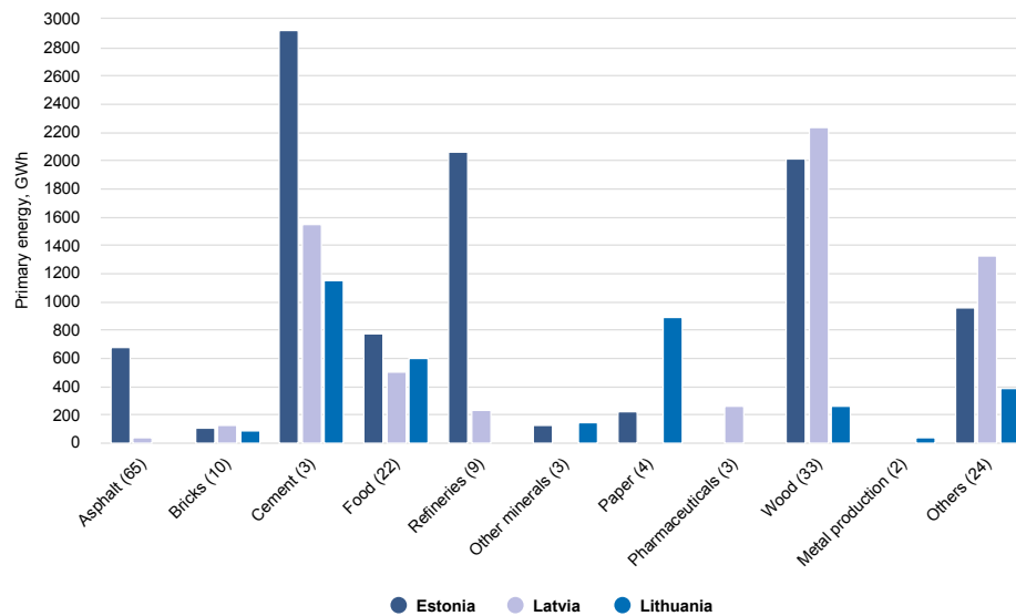
Figure 10. Annual PEC by industrial sectors (excluding chemicals) and number of sources (#)
