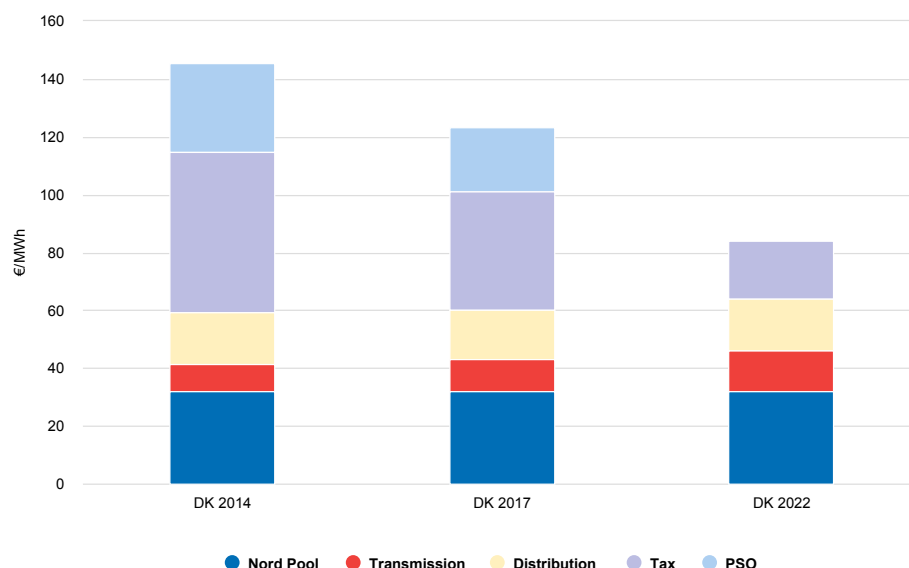
Figure 63. Electricity costs, tariffs, and taxes for electric heating in Denmark 308 309
