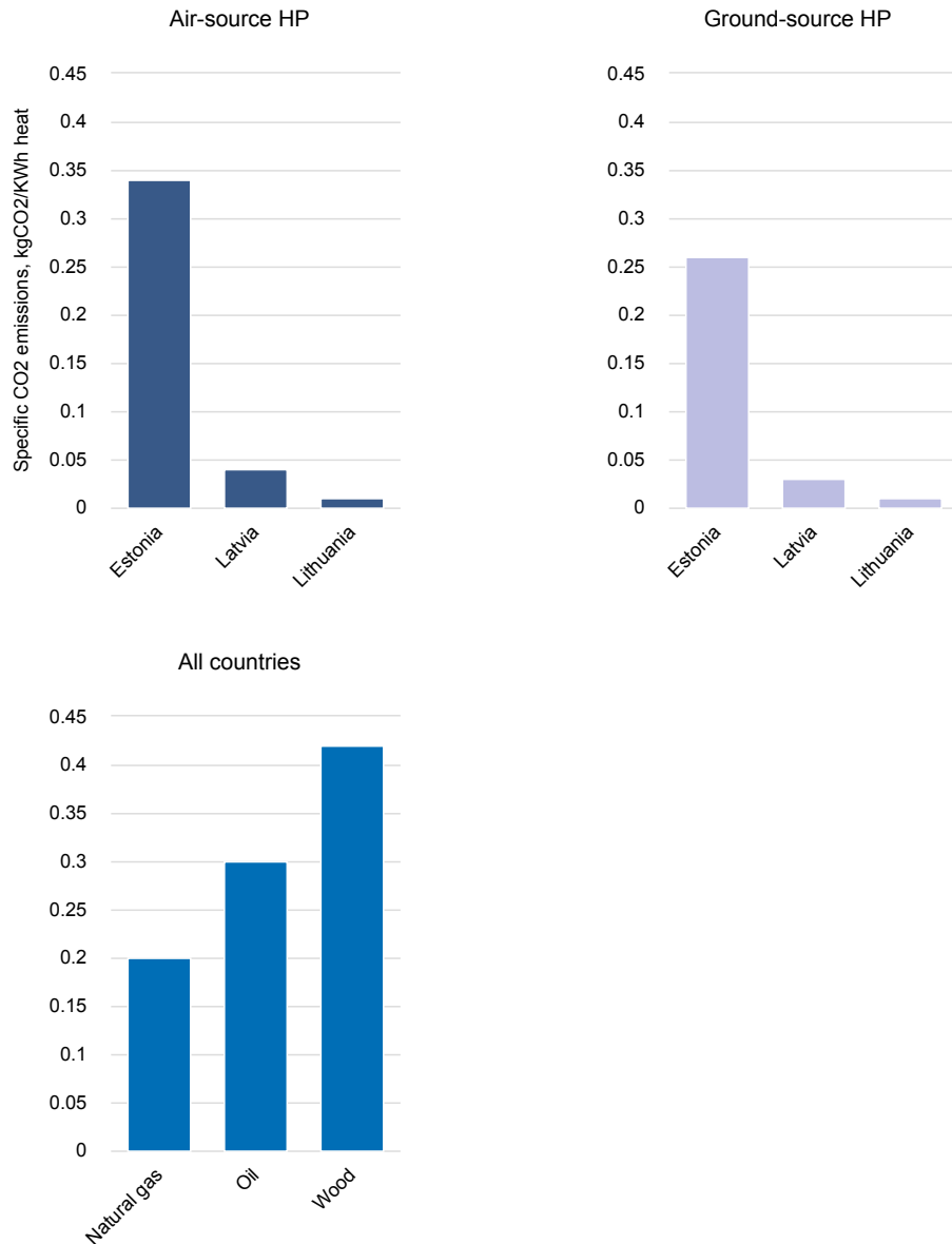
Figure 79. Specific CO 2 emissions for individual heating technologies for existing buildings in the Baltic states (*CO 2 emissions from biofuel combustion can be considered zero)
