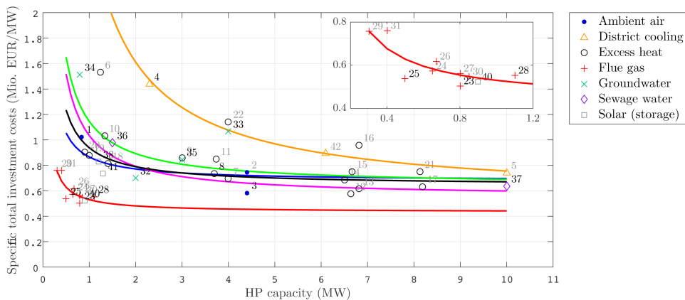
Figure 31. Specific investments for HP projects based on the heat source (copied from 231 )
