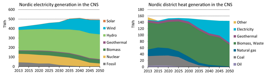
Figure 23. Nordic electricity generation and heat production, 2013 – 2050 (copied from 183 )
