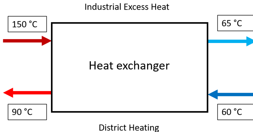
Figure 15. Industrial excess heat used by direct heat exchange to supply DH
