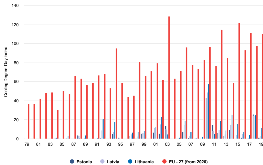
Figure 71. Annual Cooling Degree-Day Index for the Baltic states and the EU's average
