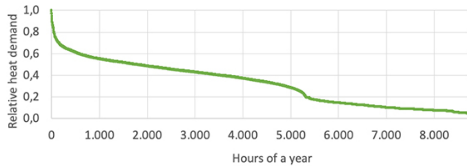
Figure 94. Load duration curve of relative hourly heat demand profiles
