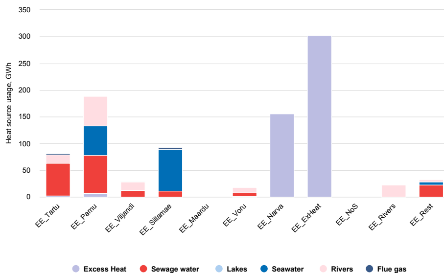
Figure 43. Use of heat sources in Estonia (without Tallinn) in 2050 according to the Base scenario
