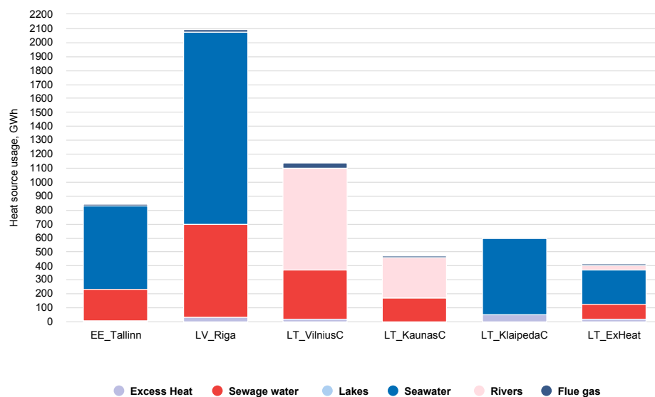
Figure 41. Use of heat sources in major DH areas in 2050 according to the Base scenario
