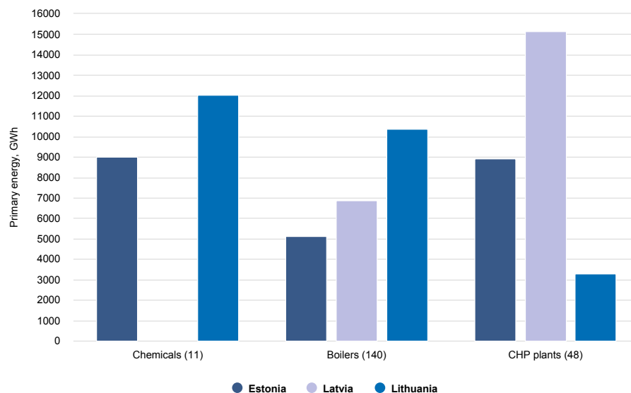
Figure 11. Annual PEC by heat production plants and the chemical sector and number of sources (#)
