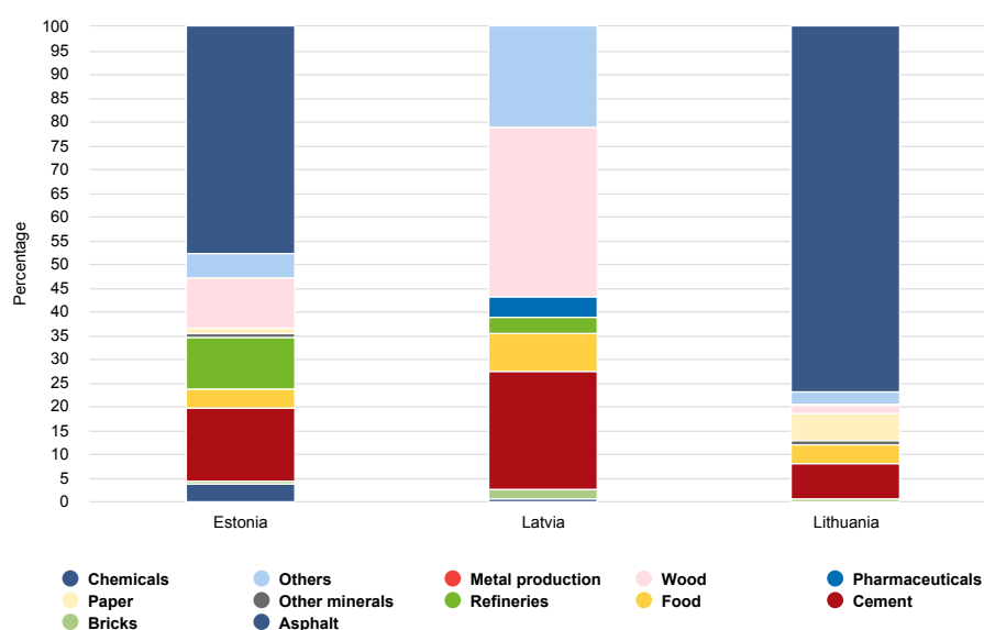
Figure 87. Proportion of industrial sectors on the PEC of 18.9, 6.3 and 15.6 GWh in Estonia, Latvia and Lithuania
