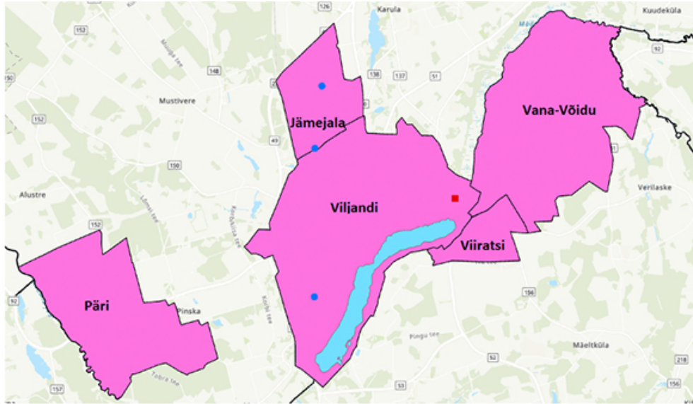
Figure 20. DH area and available heat sources around Viljandi, Estonia
