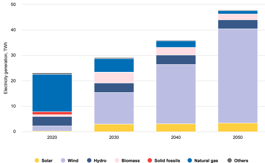
Figure 34. Electricity generation mix over the modelled period in the Baltic countries
