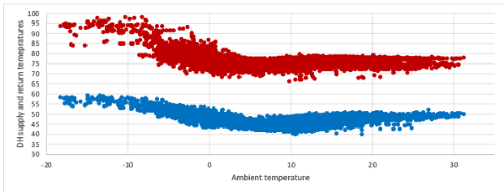
Figure 90. Measured DH supply and return temperatures of a network in Estonia in 2019
