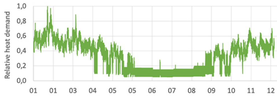
Figure 93. Relative hourly heat demand profiles
