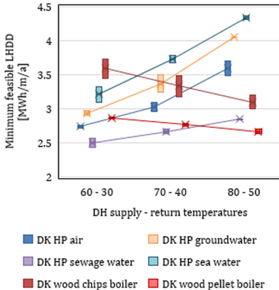
Figure 83. Minimum feasible LHDD for DH compared to individual air-source HPs (copied from 364 )
