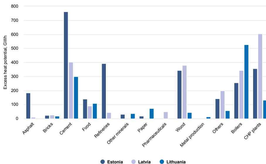
Figure 19. Theoretical excess heat potential of high-temperature heat sources
