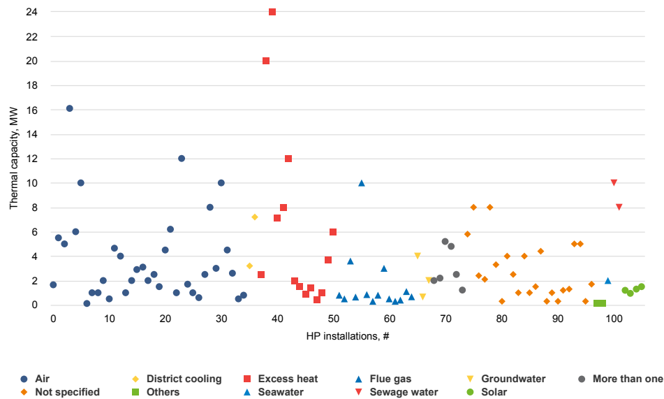
Figure 62. Installed large-scale HPs in Denmark based on the heat source used 282
