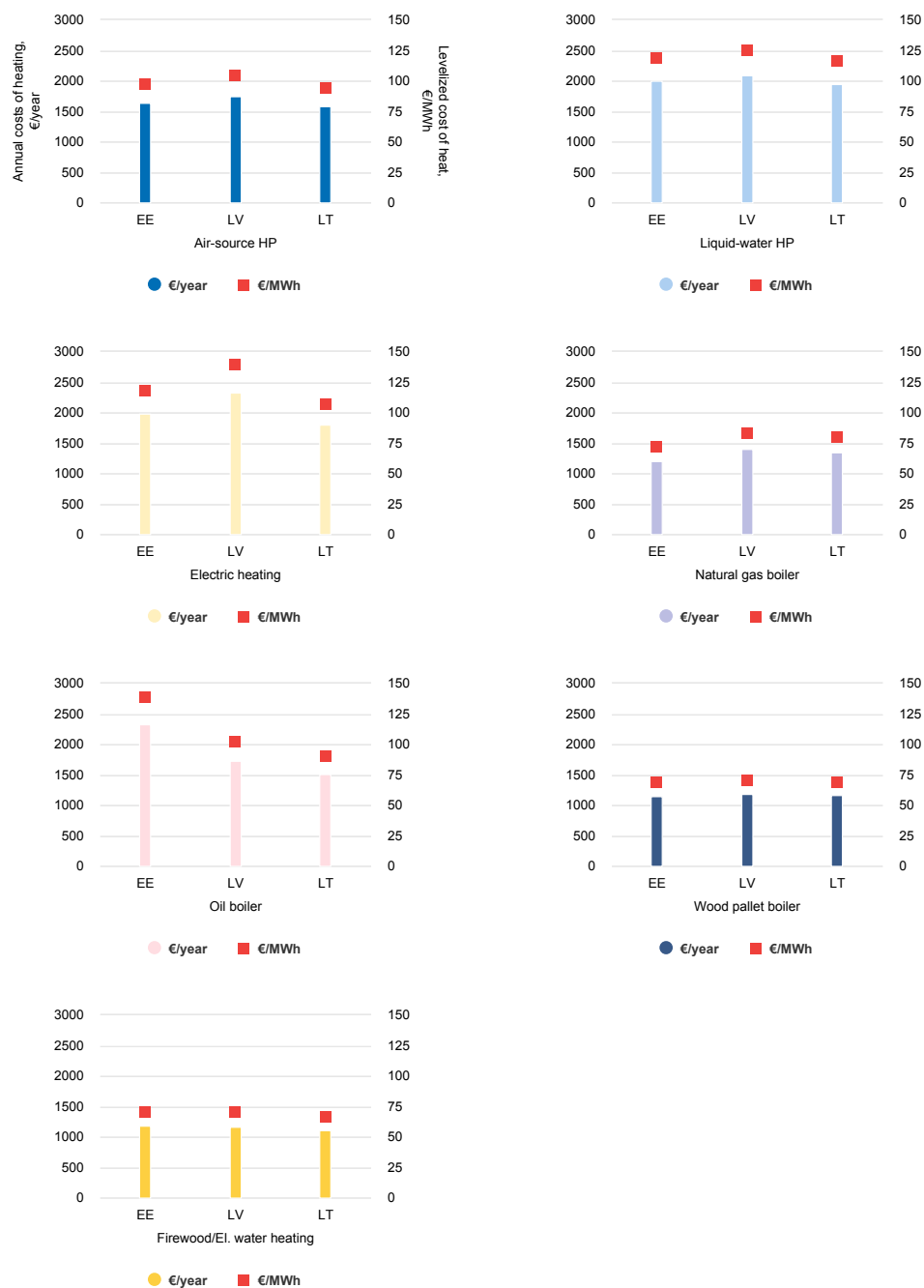
Figure 75. Heat costs for individual technologies in the Baltic states 348
