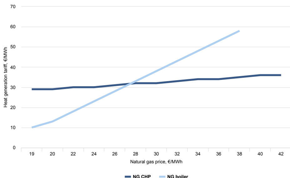
Figure 85. Heat generation tariff based on the price of natural gas for a natural gas boiler and CHP plant in Latvia 369
