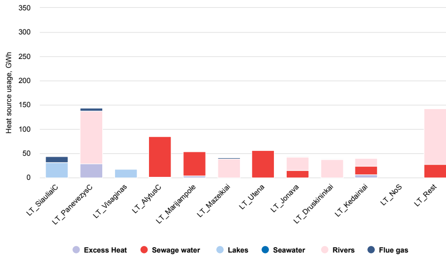
Figure 47. Use of heat sources in Lithuania (without Vilnius, Kaunas, Klaipėda, and aggregate excess heat areas) in 2050 according to the Base scenario
