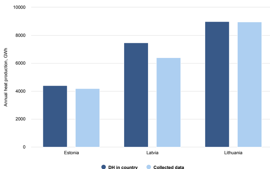
Figure 8. Annual heat production of the DH areas with collected data and total DH production
