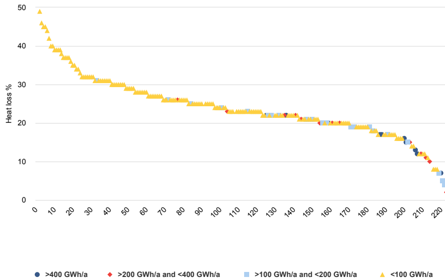
Figure 66. Heat loss in Danish DH networks in 2013/2014 315
