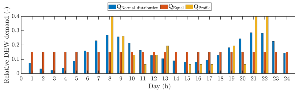
Figure 92. Domestic hot water demand for a single day
