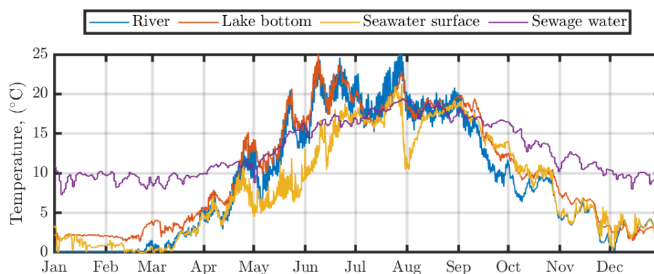
Figure 13. Heat source temperatures
