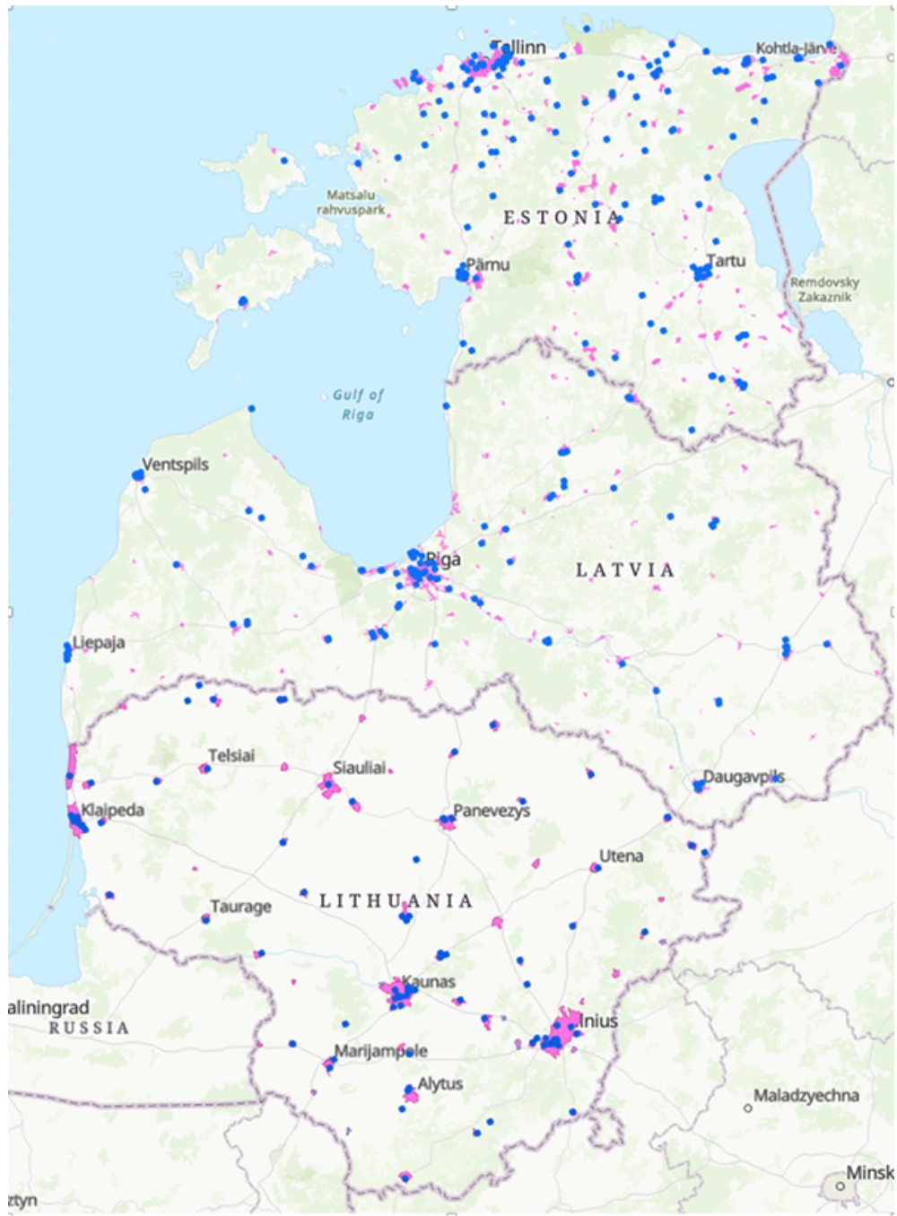
Figure 12. High-temperature heat sources (blue dots) and DH areas (in pink)
