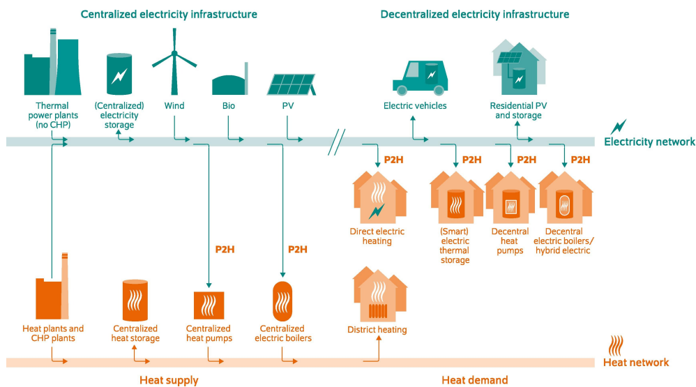
Figure 49. Centralised and decentralised (individual) P2H technologies 237
