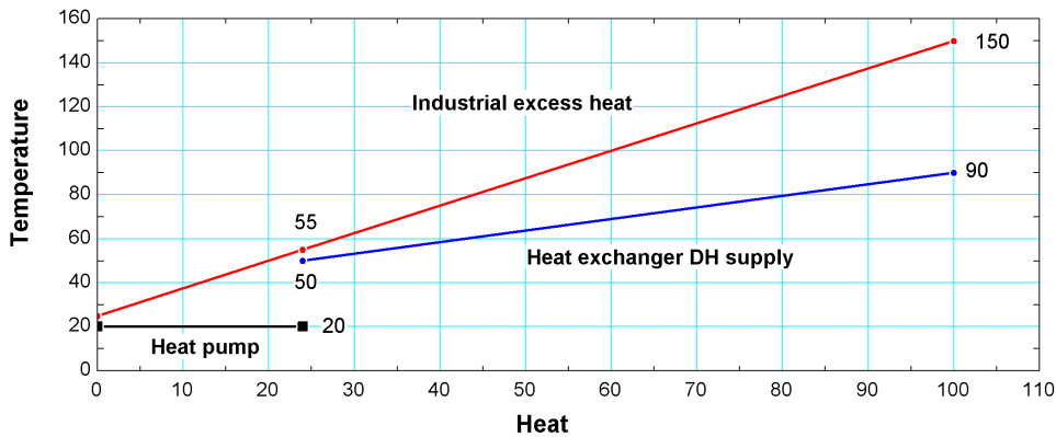
Figure 16. T-Q diagram of the utilisation of industrial excess heat by direct heat exchange and HP
