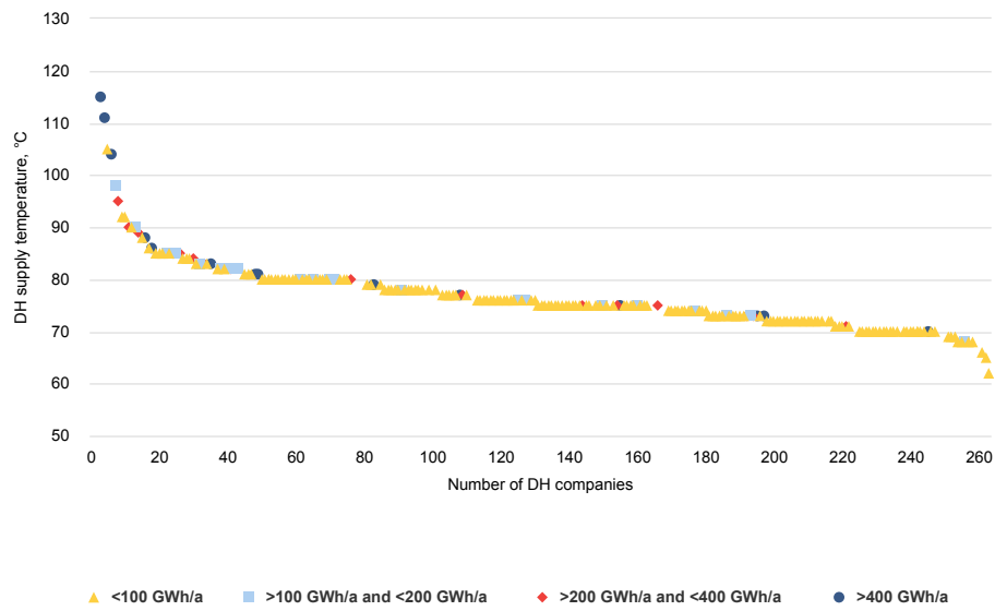
Figure 65. DH supply temperature in winter in Danish DH networks in 2013/2014 314
