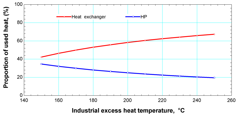
Figure 17. Proportion of heat used for the heat exchanger and HP depending on the industrial excess heat temperature
