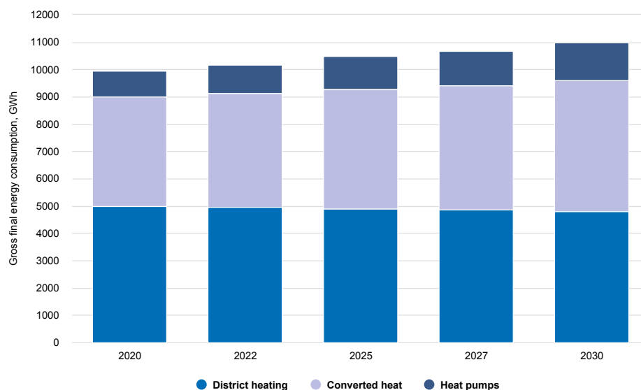
Figure 29. Renewable energy consumption in the heating sector in Estonia 189
