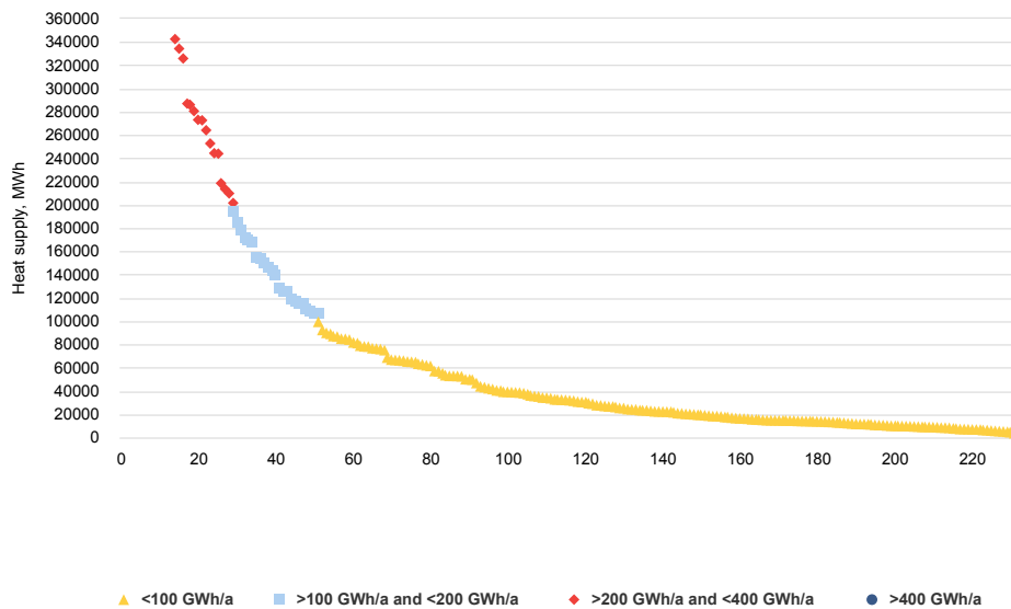
Figure 64. Heat delivered to the DH network in 2013/2014 in Denmark 313
