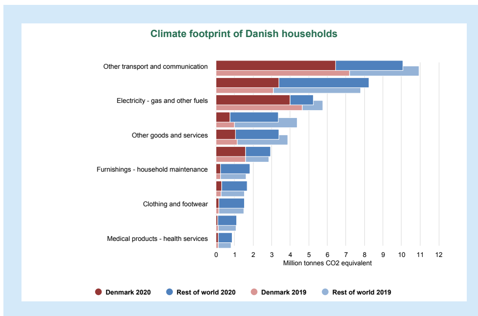
Figure 9.4. Climate footprint of Danish household consumption expenditure by types of use, 2020.
