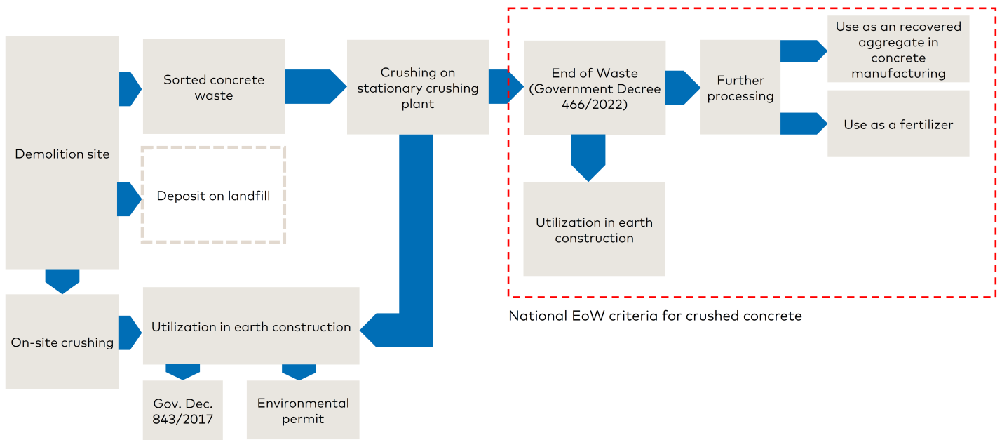
Figure 7. Recycling scheme for concrete waste according to Finnish legislation.
